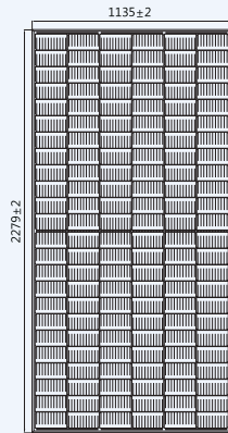
Dimensions of PV Module (Unit: mm)
