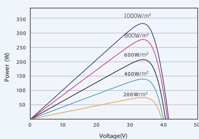
P-V Curves of PV Module (335W)
